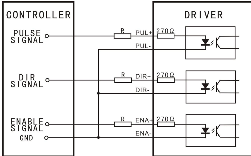
Figure1: Common-Cathode
