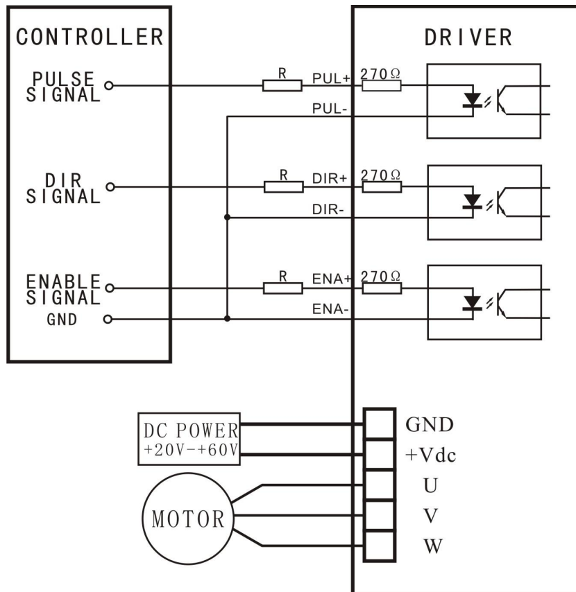
Figure 3: Typical connection
