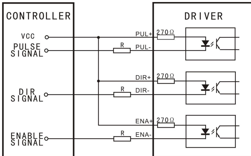
Figure2: Common-Anode
